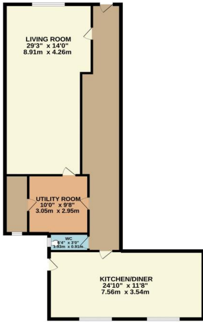
GROUND FLOOR 1055 sq.ft. (98.0 sq.m.) approx.
